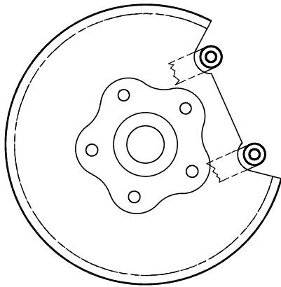
SPLASH GUARD BEFORE MODIFICATION
