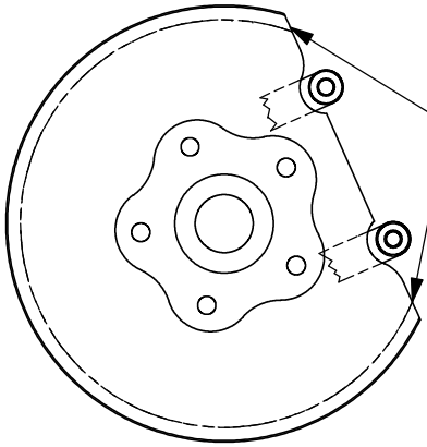
SPLASH GUARD AFTER MODIFICATION
